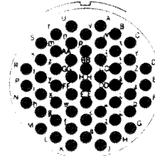
23-55 55 SIZE 20 CONTACTS
