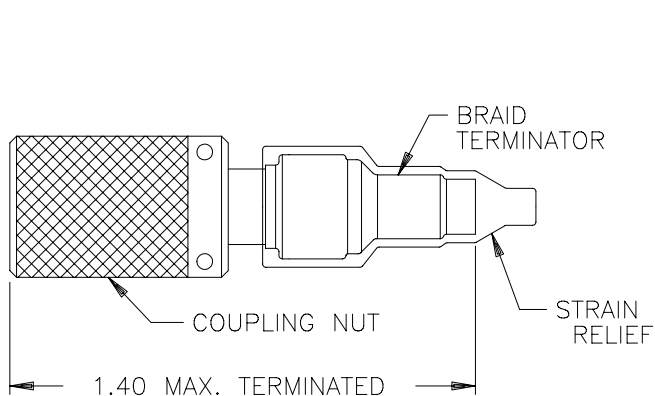
PLUG ASSEMBLY: D-621-0011
