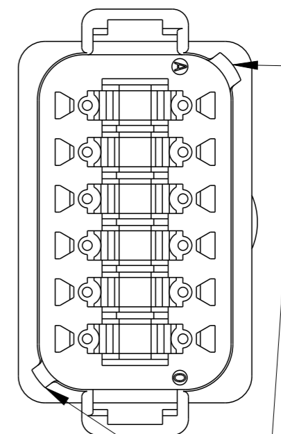
DT04-12PD-CE04 KEY -D- HOUSING COLOR: BROWN CAP COLOR: BLACK
