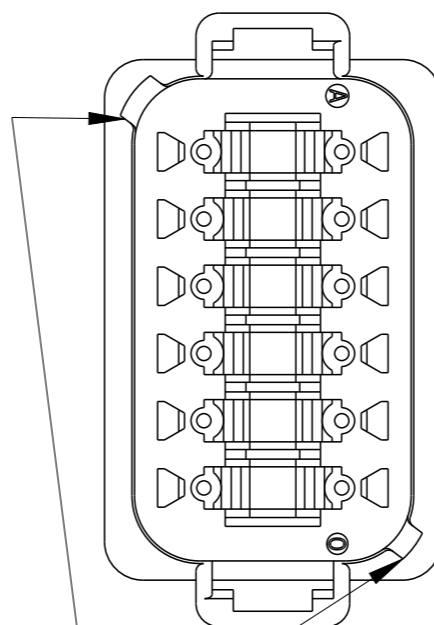
DT04-12PC-CE04 KEY -C- HOUSING COLOR: GREEN CAP COLOR: BLACK
