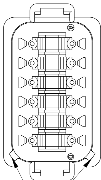
DT04-12PB-CE04 KEY -B- HOUSING AND CAP COLOR: BLACK
