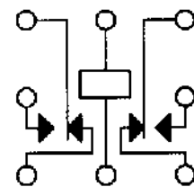
TERMINAL VIEW
