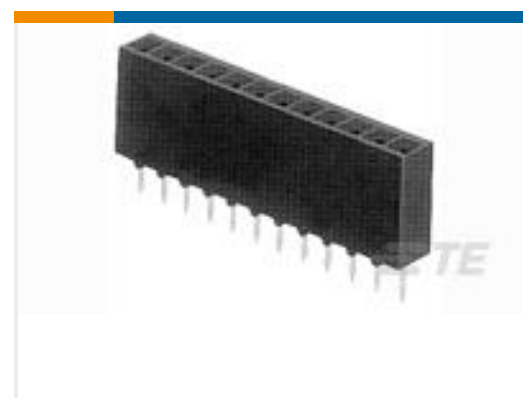
TE Part #5-87879-8 13 MODIV VRT SR OE 100 /115, ROHS
