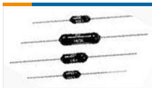
TE Part #1879665-5 H8 13K7 0.1% 15PPM
