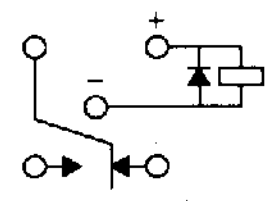
TERMINAL VIEW
