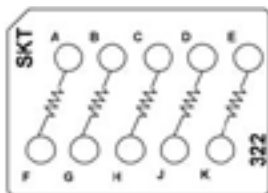
CTJ420E322 Five 4.7 k \Omega Resistors, 1/2 W
