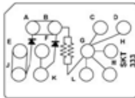
CTJ420E333 Two 2 k \Omega Resistors, 1/4 W Two JANTX 1N6677-1 Diodes
