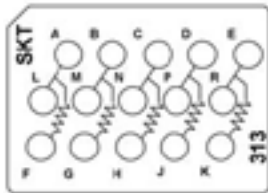
CTJ420E313 Five 100 k \Omega Resistors, 1/4 W
