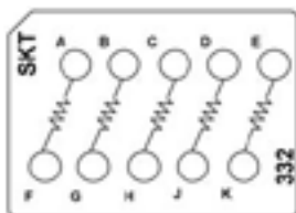
CTJ420E332 Five 10 k \Omega Resistor, 1/10 W
