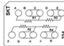
CTJ420E334 Two 10 k \Omega Resistors, 1/8 W Two 3 k \Omega Resistors, 1/8 W
