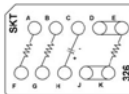
CTJ420E326 One 100 \Omega Resistor, 1/4 W One 300 \Omega Resistor, 1/4 W One 573 \Omega Resistor, 1/4 W One 10 \mu F Capacitor, 35 WVDC
