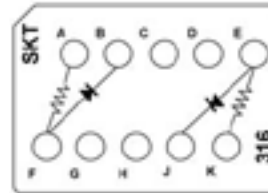
CTJ420E316 Two 1 k \Omega Resistors, 1/2 W Two 1N4007 Diodes
