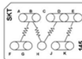
CTJ420E145 Two 100 k \Omega Resistors, 1/4 W Two 7.5 k \Omega Resistors, 1/4 W
