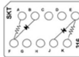
CTJ420E316 Two 1 kΩ Resistors, 1/2 W Two 1N4007 Diodes
