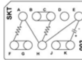
CTJ420E003 Two 150 Ω Resistors, 1/4 W One 10 μF Capacitor, 35 WVDC
