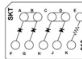
CTJ420E013 Four JANTX 1N5618 Diodes One 200 Ω Resistor, 1/8 W
