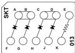
CTJ420E013 Four JANTX 1N5618 Diodes One 200 Ohm Resistor, 1/8 W
