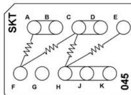
CTJ420E045 Two 40 k Resistors, 1/10 W Two 50 k Resistors, 1/10 W
