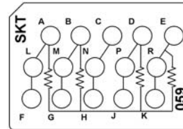
CTJ420E059 Four 150 Ohm Resistors, 1/4 W
