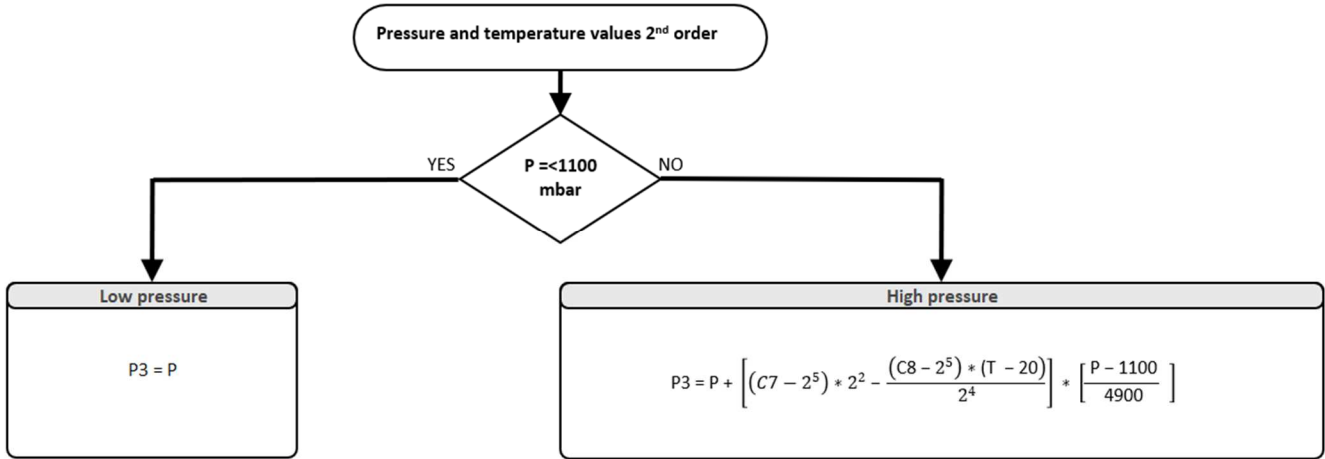
Figure 18: Flow chart for High pressure P3 calculation
