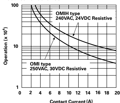
Electrical endurance
