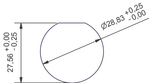
RECOMMENDED PANEL CUT-OUT DIMENSIONS
