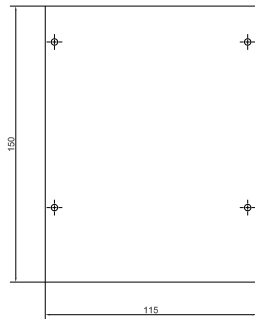
PCB MAX SIZE
