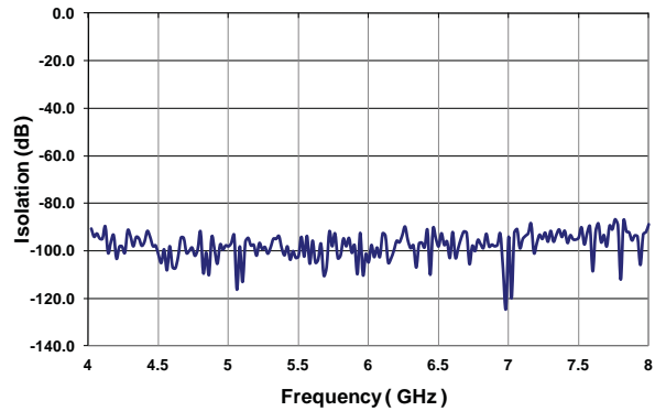
Isolation (4-8 GHz)
