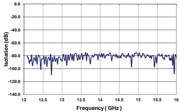
Isolation (12-16 GHz)
