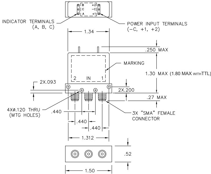
Standard Width Body
