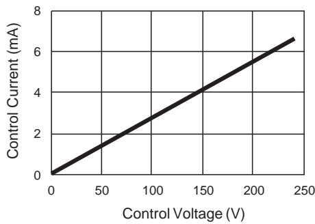
Figure 3b — DRXXA25 relays
