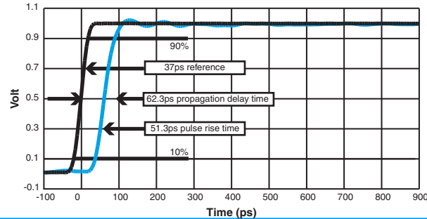
GRF300 Time Response (RF Note 6)
