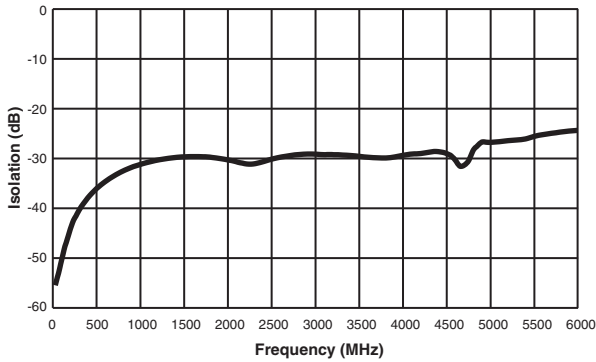
Isolation Across Contacts (RF Note 4)
