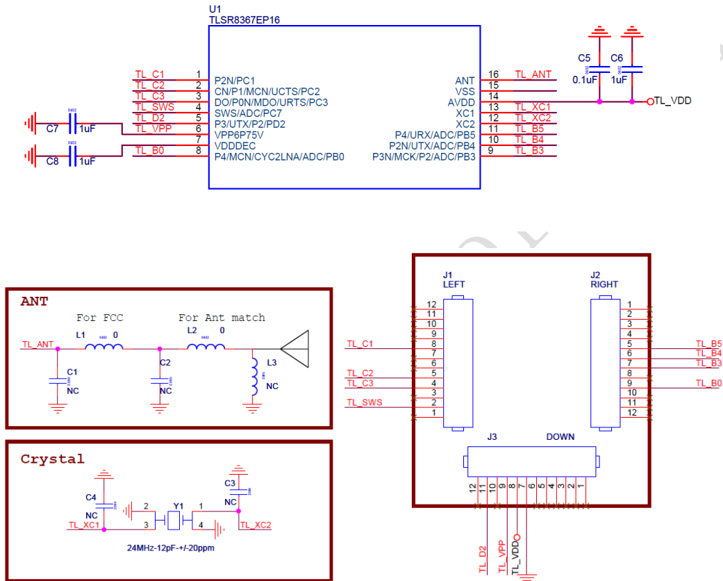
Figure 15- 1 Schematic for TLSR8367EP16
