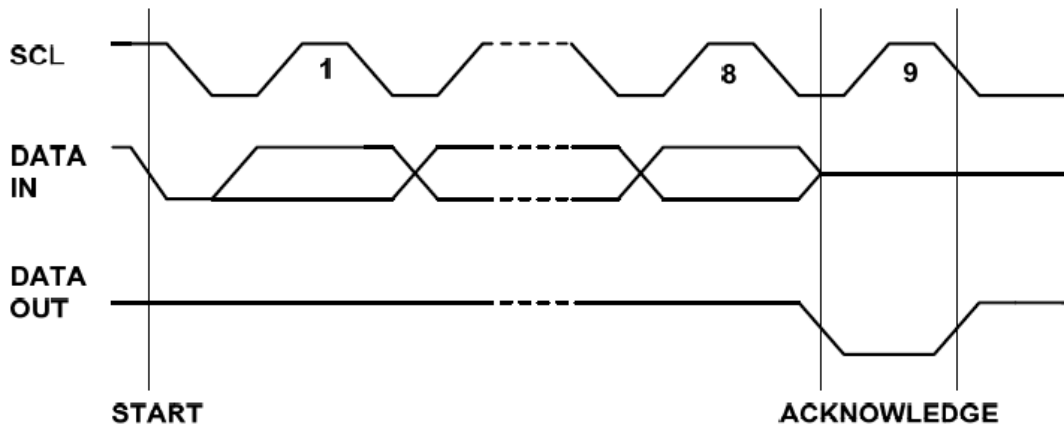
Figure 12- 3 Send Ack
