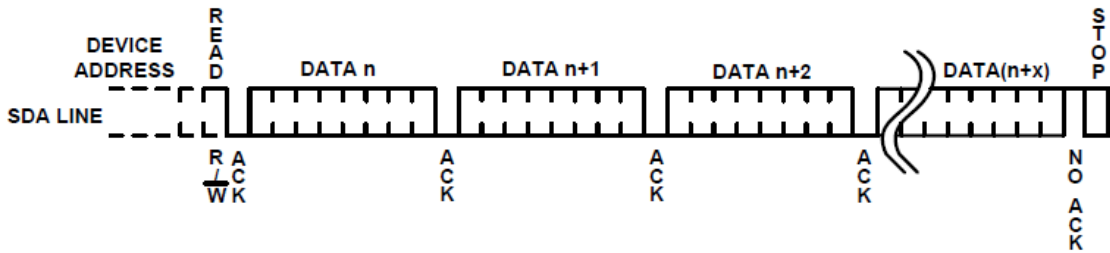
Figure 12- 9 Sequential read
