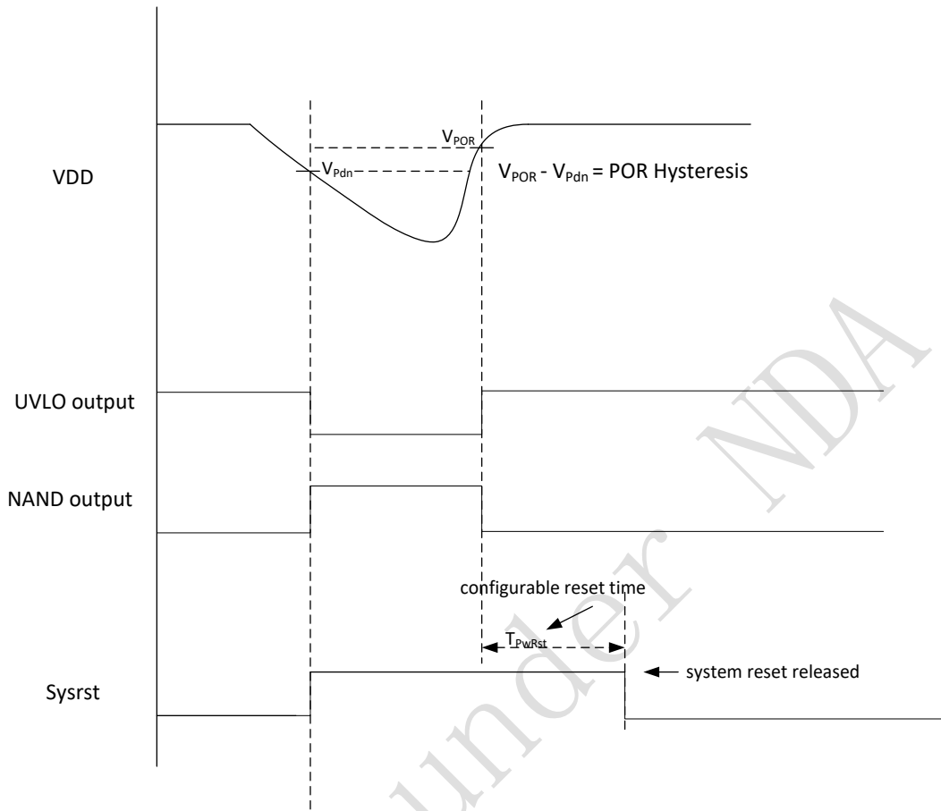
Figure 2- 6 Power-down sequence
