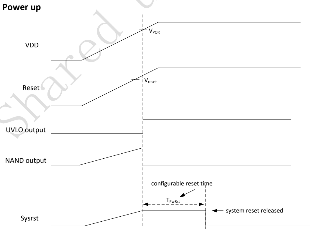
Figure 2- 5 Power-up sequence
