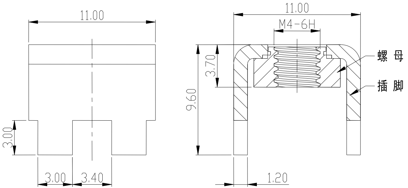
外形尺寸 (Shape Dimension)
