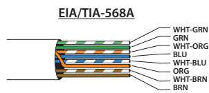
RJ45 Cable Connection
