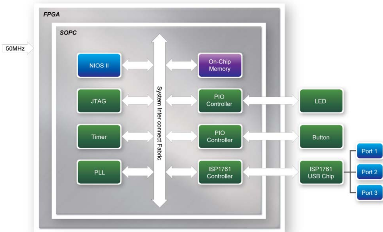
Figure 5.2. Hardware Block Diagram of the USB-Host Demonstration
