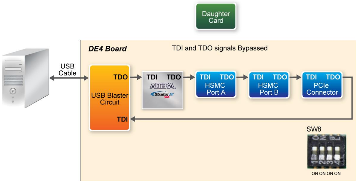
Figure 2–16 JTAG chain for a daughter card (JTAG not used) connected to HSMC port A of the DE4
