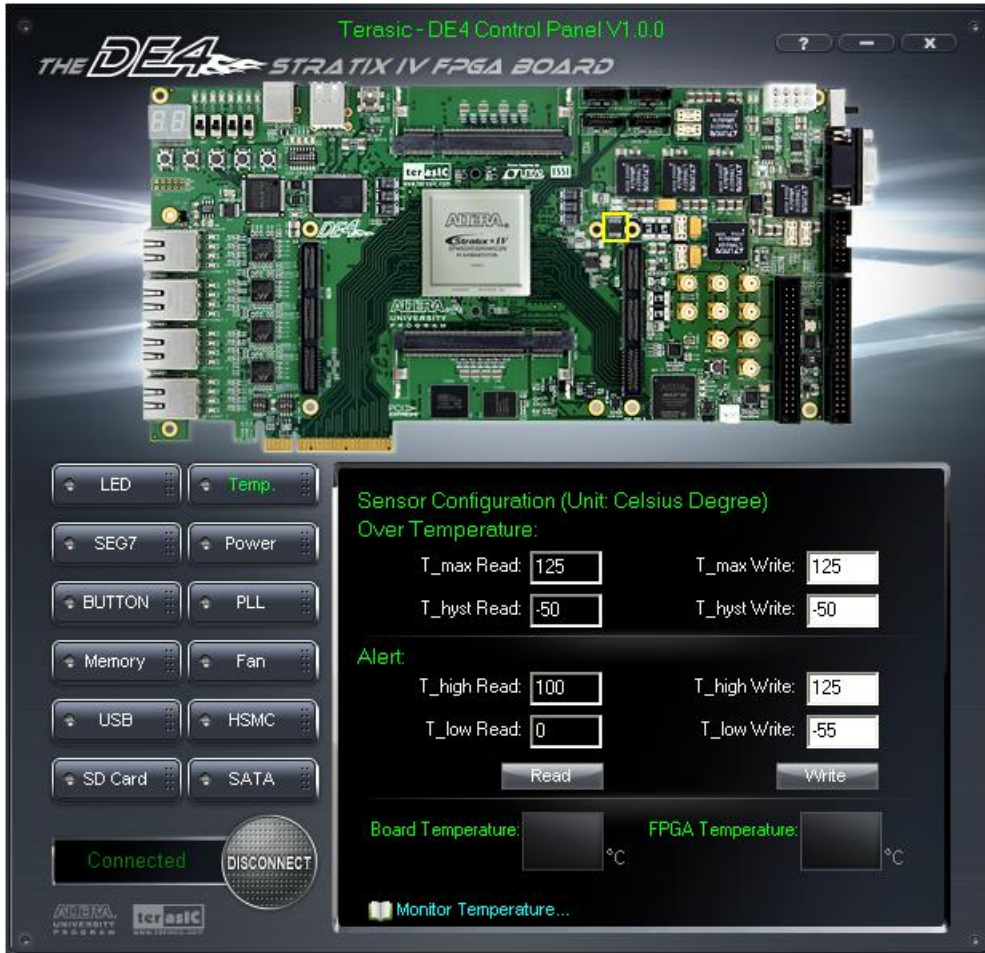
Figure 3–12 Accessing the Temperature Sensor through Control Panel
