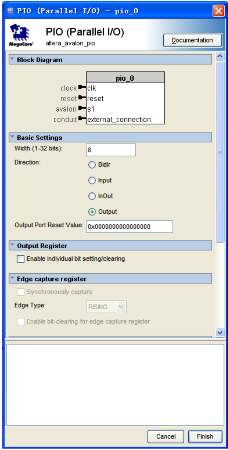
Figure 7-31 Add PIO
