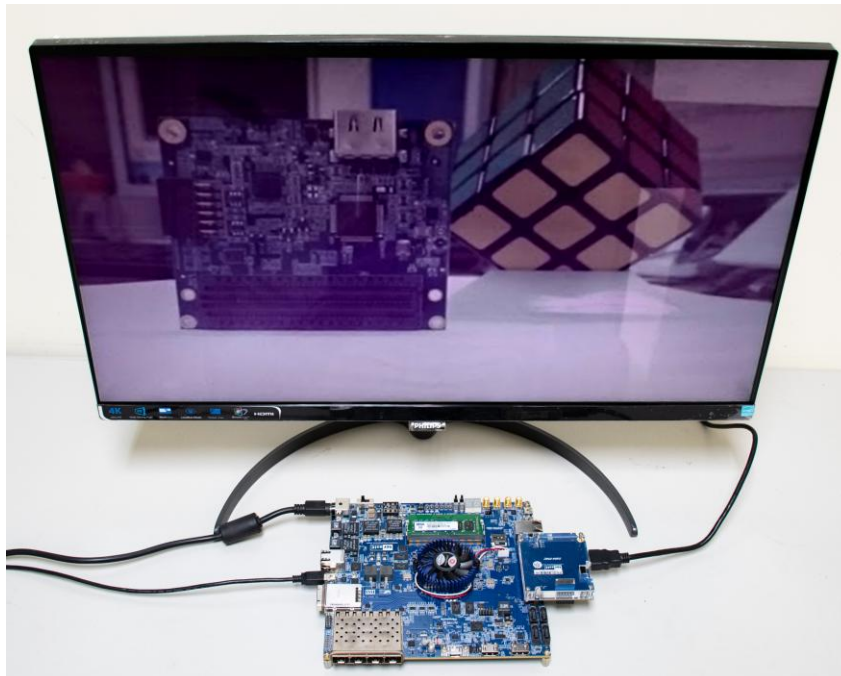
Figure 4-12 HAN demo hardware setting up
