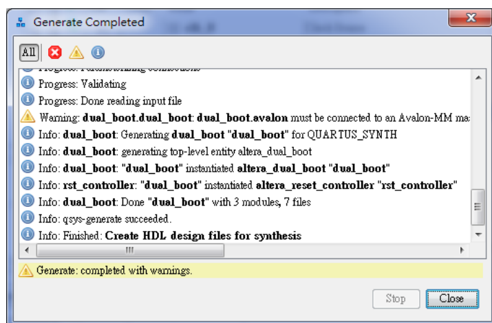
Figure 6-9 Generate completed.
