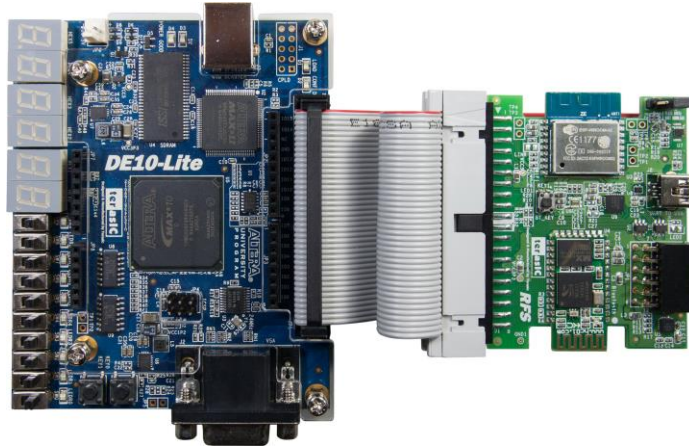
Figure 4-18 Setup HC-05 Configuration Demo to DE10-Lite
