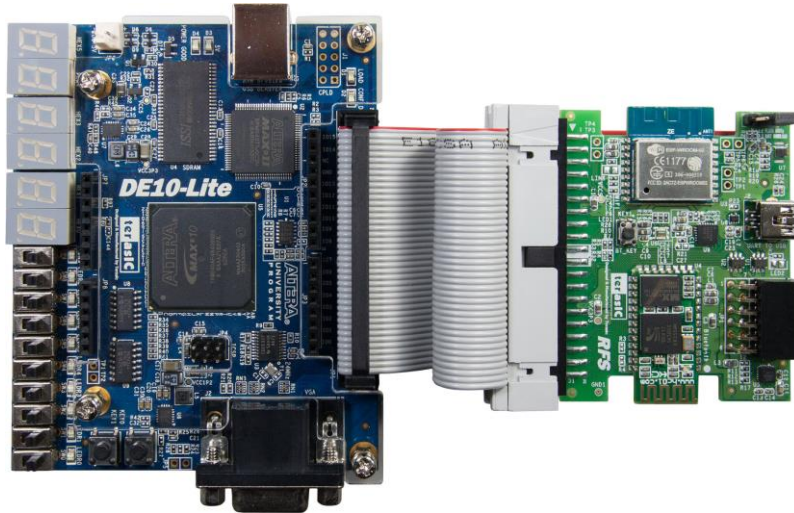
Figure 3-10 Demo setup on DE10-Lite
