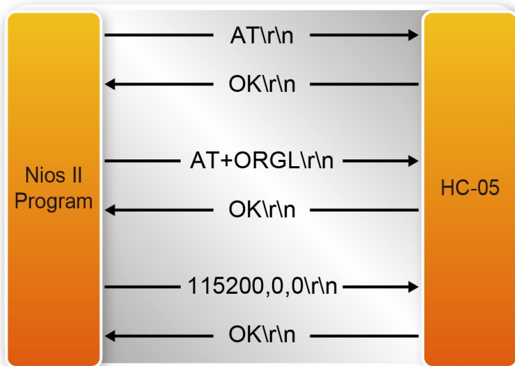
Figure 4-14 Handshake Chart
