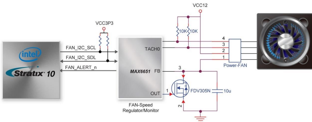
Figure 2-9 Connections between the Fan-Speed Regulator/ Monitor and the Stratix 10 GX/SX FPGA
