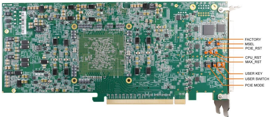
Figure 2-2 FPGA Board (Bottom)
