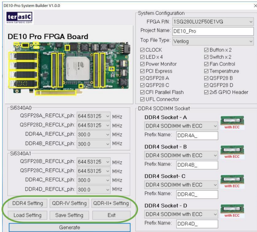
Figure 3-8 Project Settings
