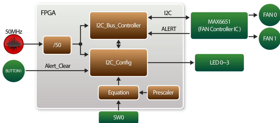
Figure 5-17 Block diagram of the fan speed control demonstration
