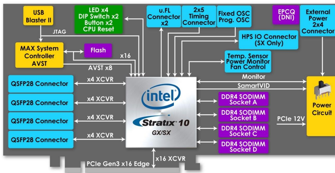
Figure 1-1 Block diagram of the DE10-Pro board
