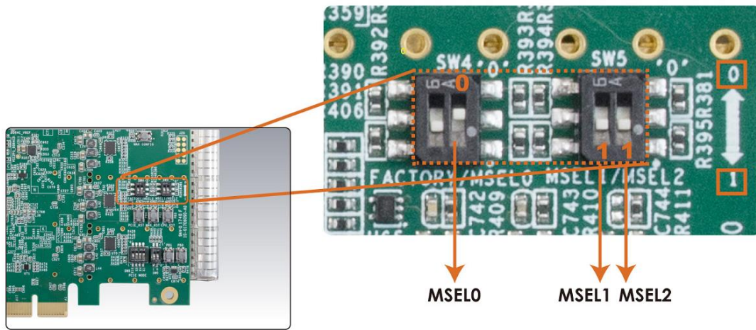
Figure 4-1 MSEL[2:0]=110
