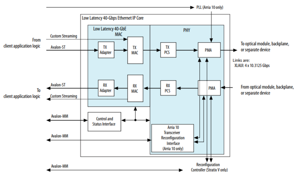
Figure 9-10 Block diagram of 40GbE demo
