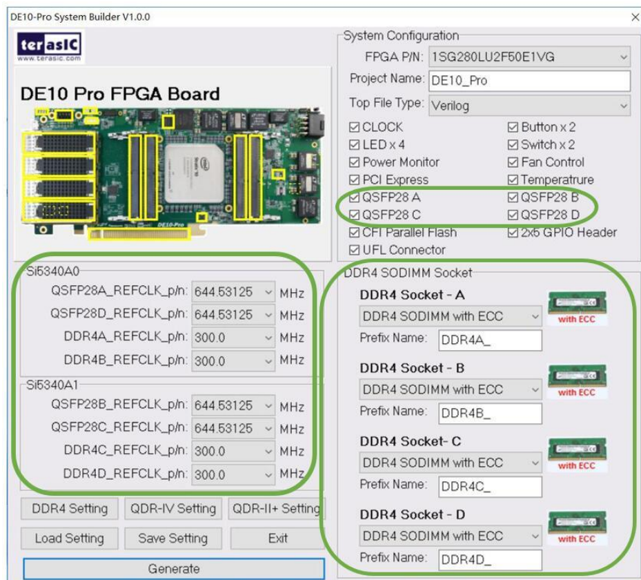
Figure 3-7 External programmable oscillators
