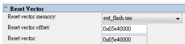
Figure 4-9 User Software Reset Vector Settings for NIOS II Processor
