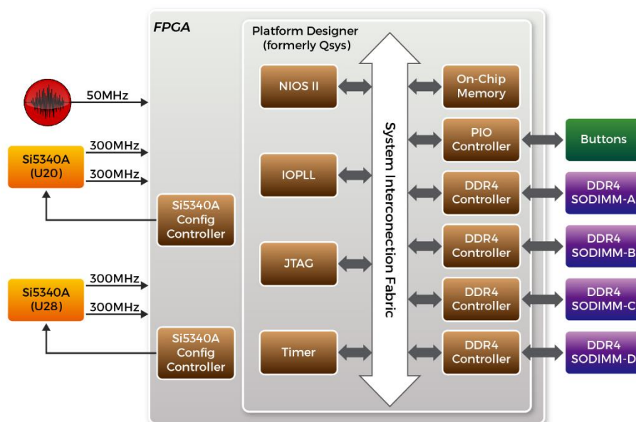
Figure 6-2 Block diagram of the DDR4 Basic Demonstration
