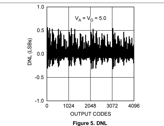
Figure 5. DNL
