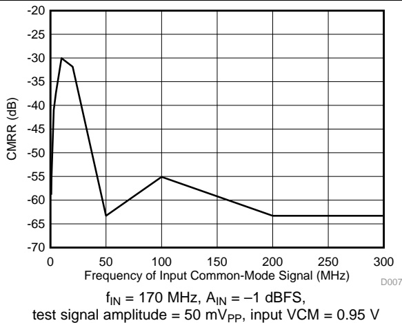
Figure 135. Common-Mode Rejection Ratio vs Test Signal Frequency
