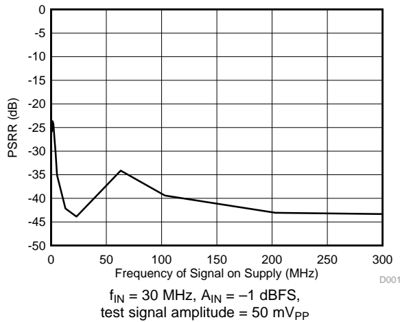
Figure 133. Power-Supply Rejection Ratio vs Test Signal Frequency
