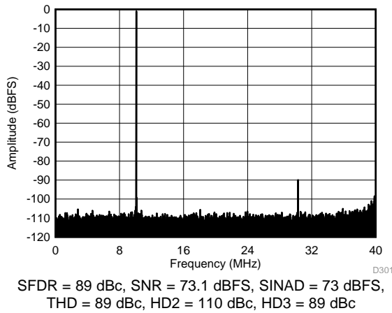
Figure 67. FFT for 10-MHz Input Signal (Chopper On, Dither On)
