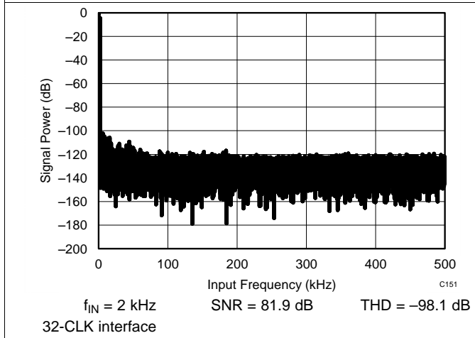
Figure 26. Typical FFT
