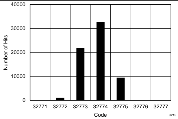
Figure 15. DC Histogram
