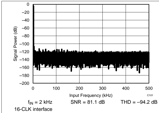
Figure 24. Typical FFT
