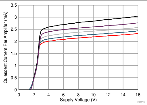
图 6-20. Quiescent Current vs Power Supply
