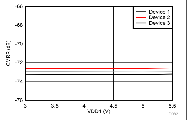
图 6-28. Common-Mode Rejection Ratio vs Supply Voltage
