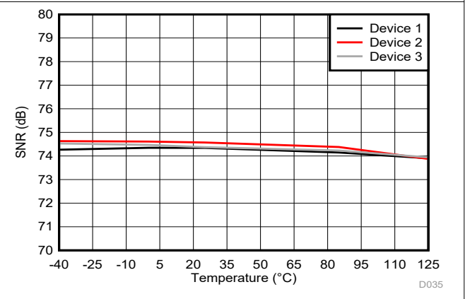
图 6-26. Signal-to-Noise Ratio vs Temperature
