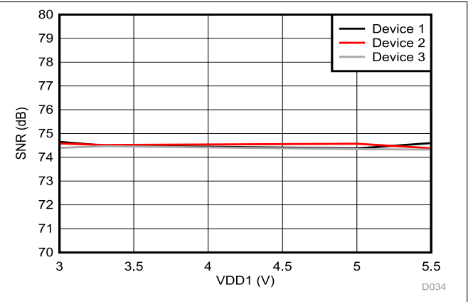
图 6-24. Signal-to-Noise Ratio vs High-Side Supply Voltage
