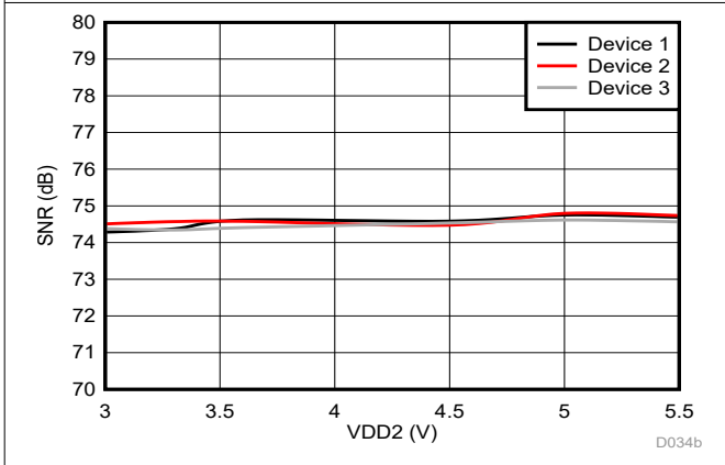
图 6-25. Signal-to-Noise Ratio vs Low-Side Supply Voltage
