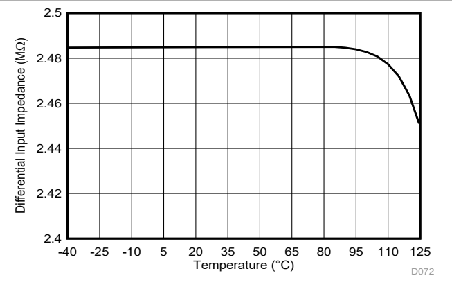
图 6-10. Differential Input Impedance vs Temperature
