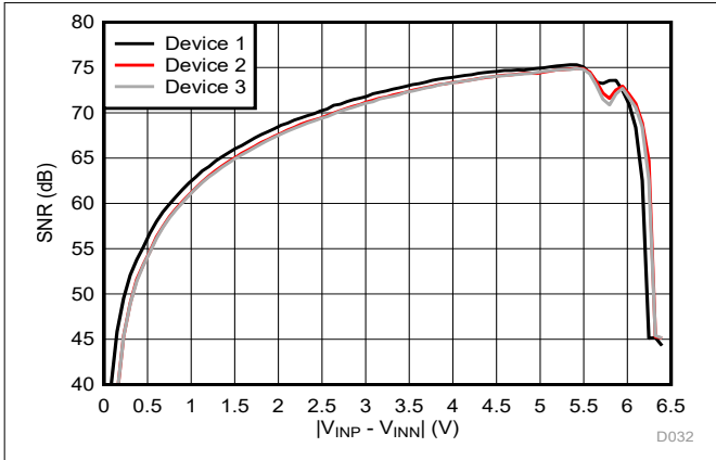
图 6-23. Signal-to-Noise Ratio vs Input Voltage
