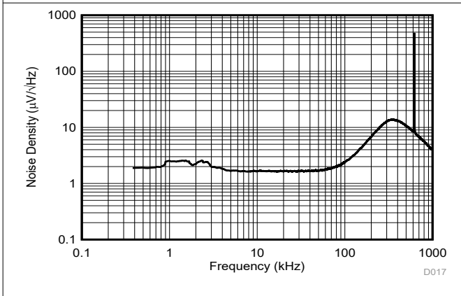
图 6-27. Input-Referred Noise Density vs Frequency
