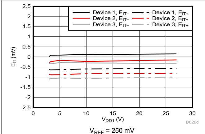
Figure 6-31. Cmp1 Trip Threshold Error vs Supply Voltage
