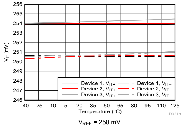
Figure 6-12. Cmp0 Trip Threshold vs Temperature
