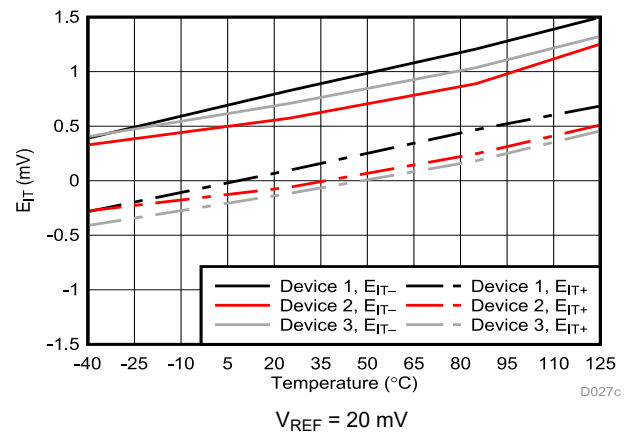
Figure 6-26. Cmp1 Trip Threshold Error vs Temperature
