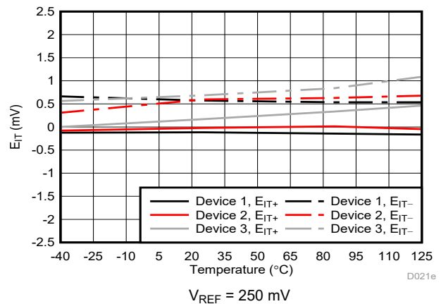
Figure 6-14. Cmp0 Trip Threshold Error vs Temperature
