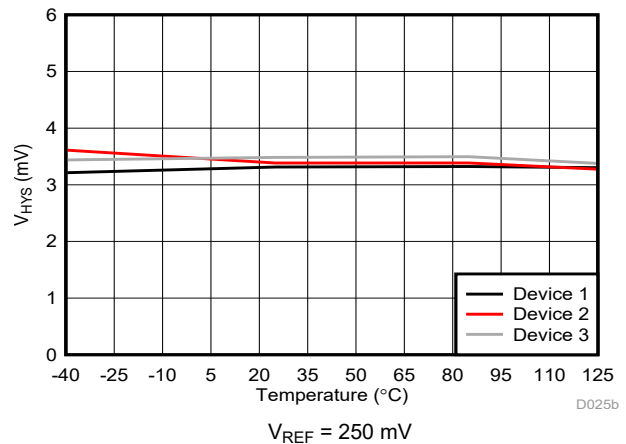
Figure 6-16. Cmp0 Trip Threshold Hysteresis vs Temperature
