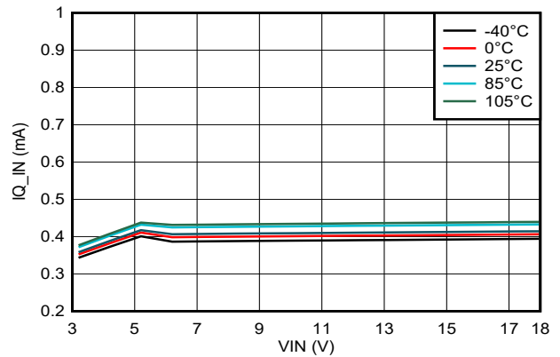
Figure 6-8. Input Quiescent Current vs. Input Voltage
