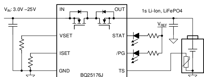
Simplified schematic
