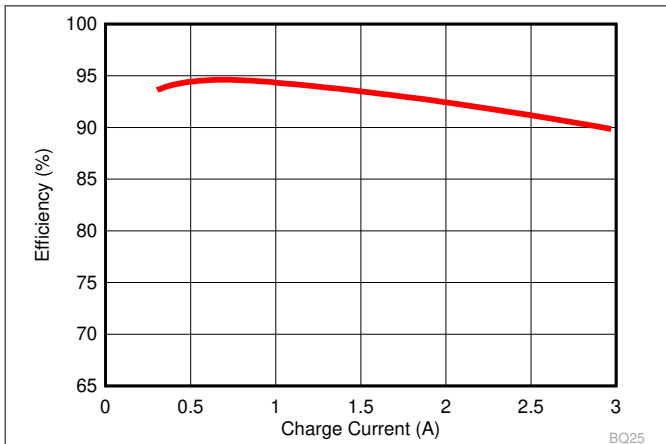
图 8-1. 1-Cell Battery Charge Efficiency vs. Charge Current
