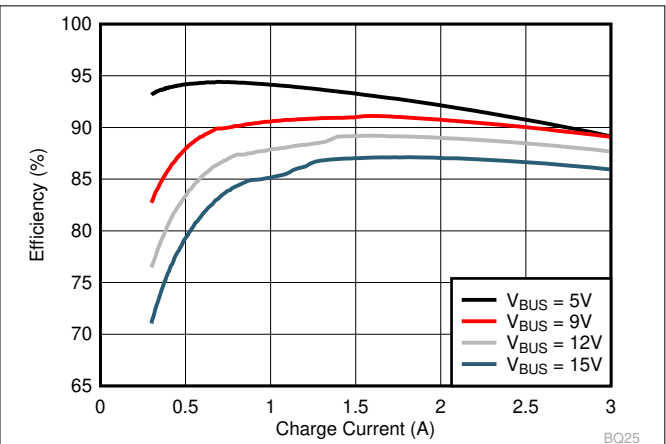
图 8-2. 1-Cell Battery Charge Efficiency vs. Charge Current
