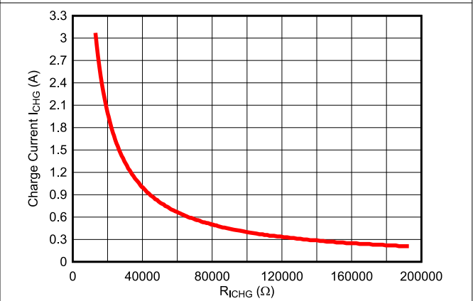
图 8-4. Charge Current vs. Charge Current Setting Resistance RICHG
