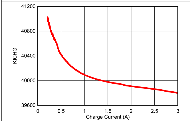
图 8-3. KICHG vs. Charge Current
