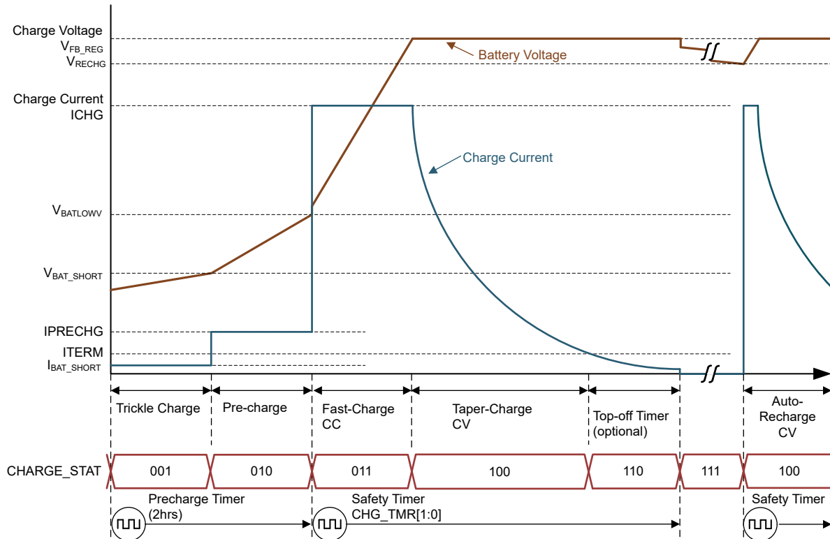
Figure 8-3. Typical Li-Ion Battery Charging Profile
