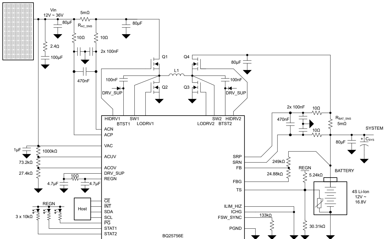
Figure 9-1. BQ25756E: Solar Charging with Autonomous MPPT Algorithm to Charge 4s Battery with Maximum 15-A Charge Current
