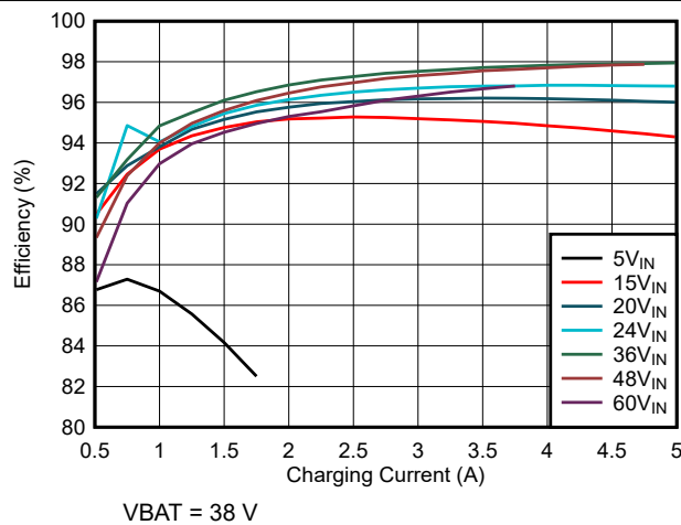
图 7-3. Charge Efficiency vs Charge Current (10s battery configuration)
