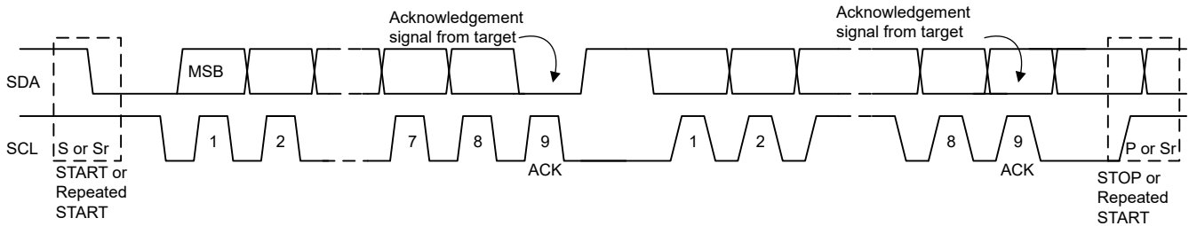
图 8-10. Data Transfer on the I 2 C Bus
