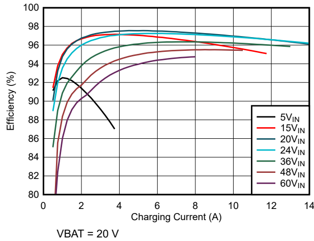
图 7-1. Charge Efficiency vs Charge Current (5s battery configuration)
