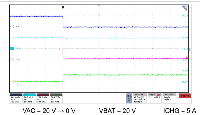
图 9-4. VAC Un-plug Power Down with 5-A ICHG
