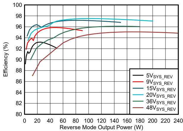
Figure 7-9. Reverse Mode Efficiency (5s battery configuration)
