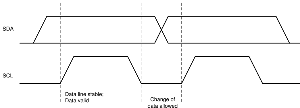
图 8-8. Bit Transfers on the I 2 C Bus
