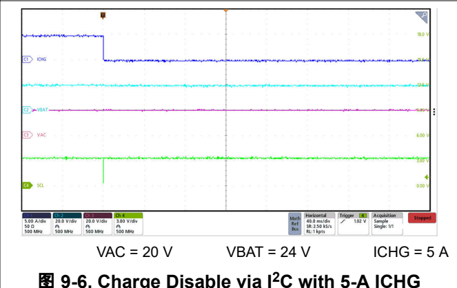
图 9-6. Charge Disable via I 2 C with 5-A ICHG
