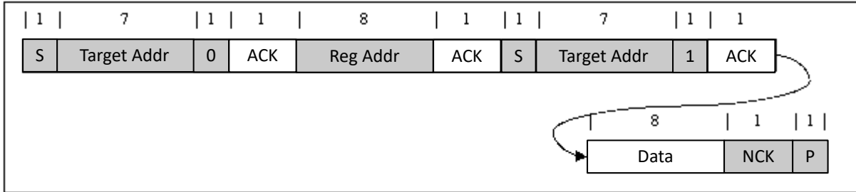
图 8-13. Single Read
