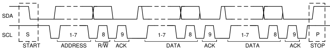
图 8-11. Complete Data Transfer on the I 2 C Bus
