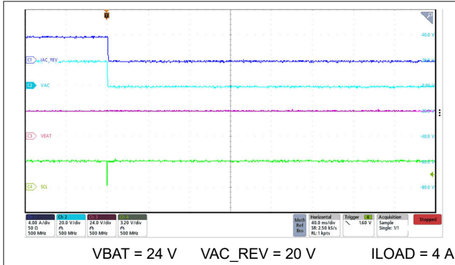
图 9-15. Reverse Mode Power Down with 4-A Load
