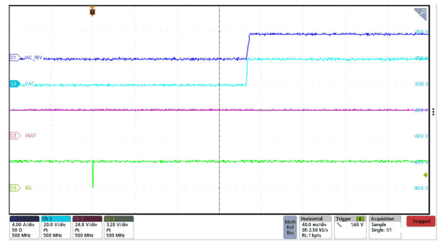
VBAT = 24 V VAC_REV = 20 V ILOAD = 4 A 图 9-14. Reverse Mode Power Up with 4-A Load
