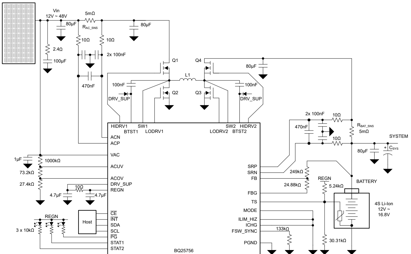
图 9-1. BQ25756: Solar Charging with Autonomous MPPT Algorithm to Charge 4s Battery with Maximum 15-A Charge Current
