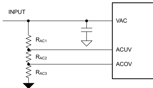
图 8-1. ACUV and ACOV Programming
