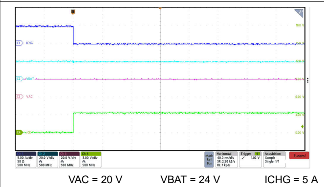
图 9-8. Charge Disable via \overline{\text{CE}} Pin with 5-A ICHG
