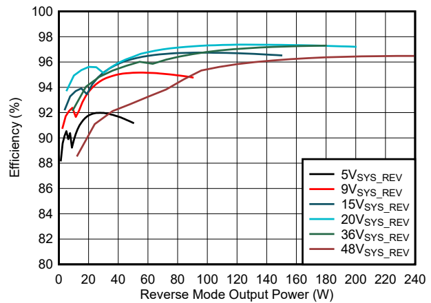
Figure 7-10. Reverse Mode Efficiency (7s battery configuration)
