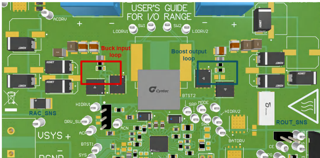
图 11-1. PCB Layout Reference Example Top View
