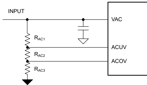
图 9-2. ACUV and ACOV Resistor Divider
