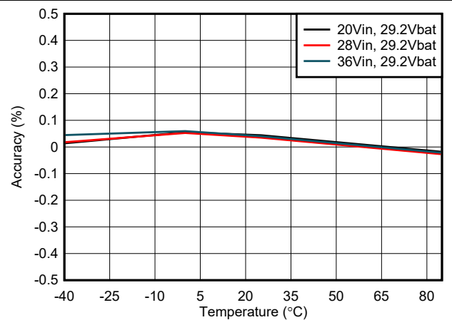
图 7-4. Charge Voltage Accuracy vs Temperature
