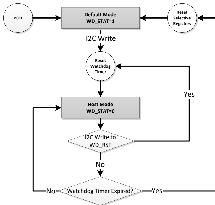
图 8-16. Watchdog Timer Flow Chart
