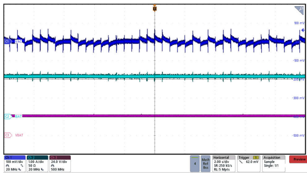
VOC = 30 V VBAT = 24 V P&O Timer = 0.5s ISC = 3.5 A 图 9-13. Max Power Point Tracking (MPPT) Perturb and Observe
