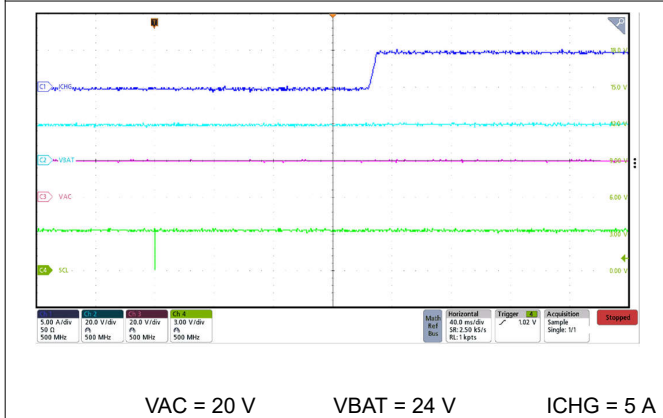
图 9-5. Charge Enable via I 2 C with 5-A ICHG
