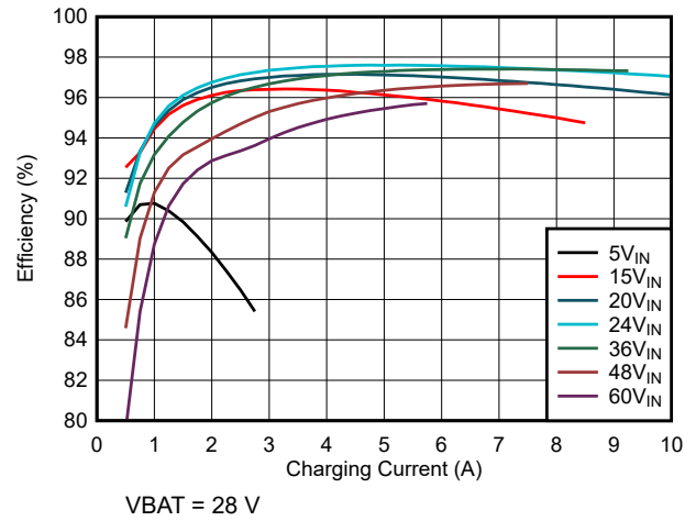
图 7-2. Charge Efficiency vs Charge Current (7s battery configuration)
