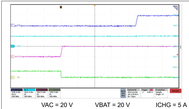
图 9-3. VAC Plug-In Power Up with 5-A ICHG
