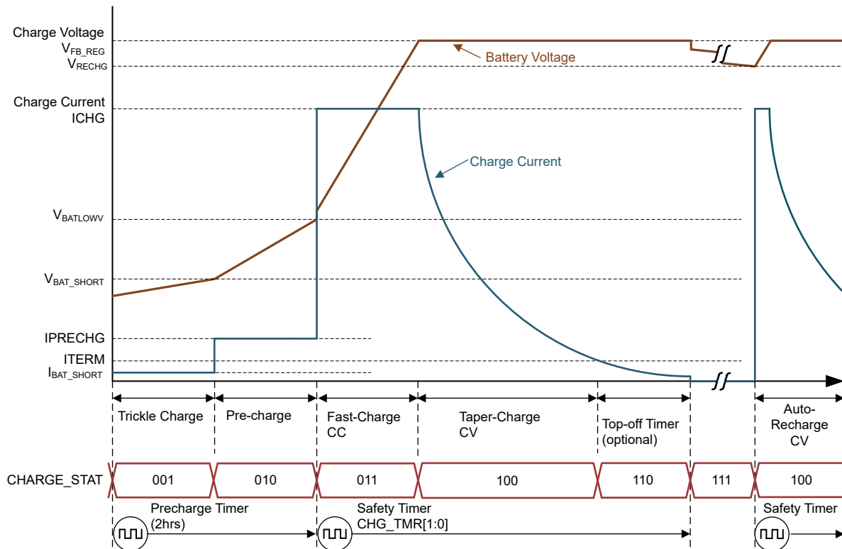
图 8-3. Typical Li-Ion Battery Charging Profile
