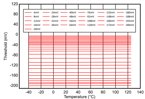
Figure 6-20. Overcurrent in Discharge Protection 1 (OCD1) Threshold vs. Temperature
