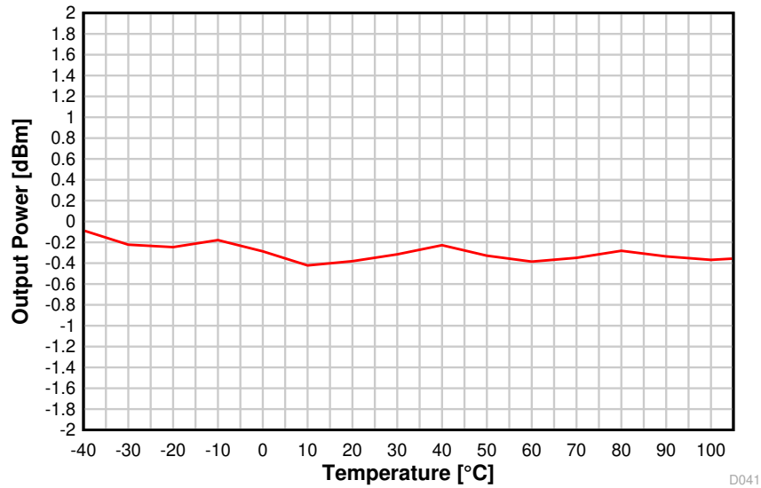
图 8-21. Output Power vs. Temperature (BLE 1 Mbps, 2.44 GHz)
