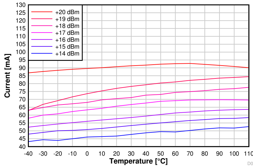
图 8-9. TX Current vs. Temperature (BLE 1 Mbps, 2.44 GHz, VDDS = 3.3 V)
