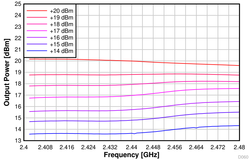
图 8-31. Output Power vs. Frequency (BLE 1 Mbps, 2.44 GHz, +20 dBm PA)
