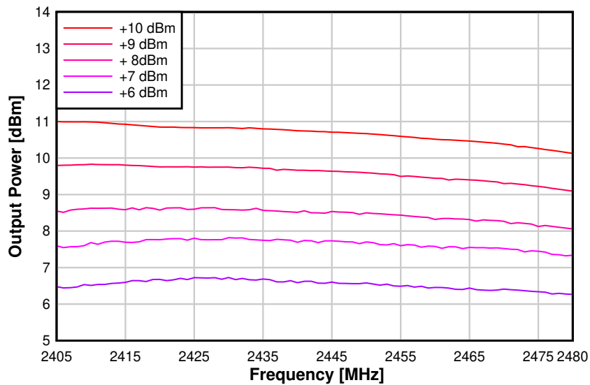
图 8-32. Output Power vs. Frequency (250 kbps, +10 dBm PA)
