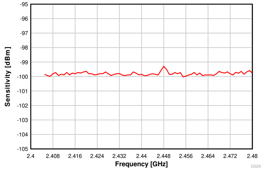
图 8-15. Sensitivity vs. Frequency (250 kbps, 2.44 GHz)
