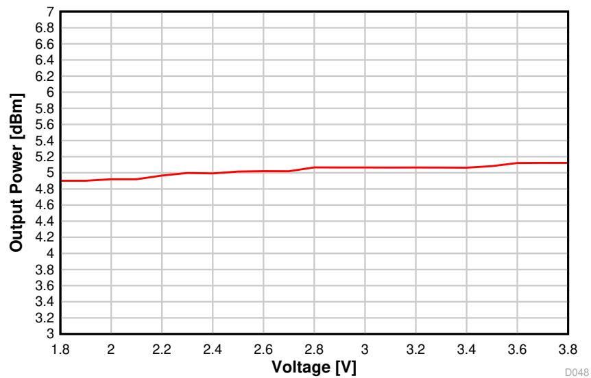
图 8-26. Output Power vs. Supply Voltage (VDD5) (BLE 1 Mbps, 2.44 GHz, +5 dBm)
