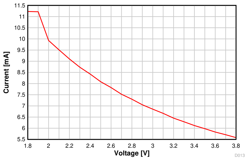
图 8-7. RX Current vs. Supply Voltage (VDDS) (BLE 1 Mbps, 2.44 GHz)
