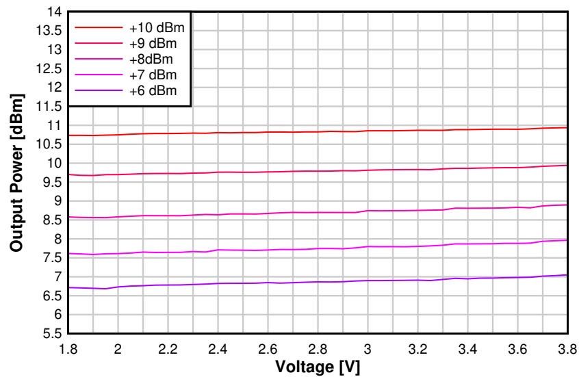
图 8-28. Output Power vs. Supply Voltage (VDDS) (2.44 GHz, +10 dBm PA)
