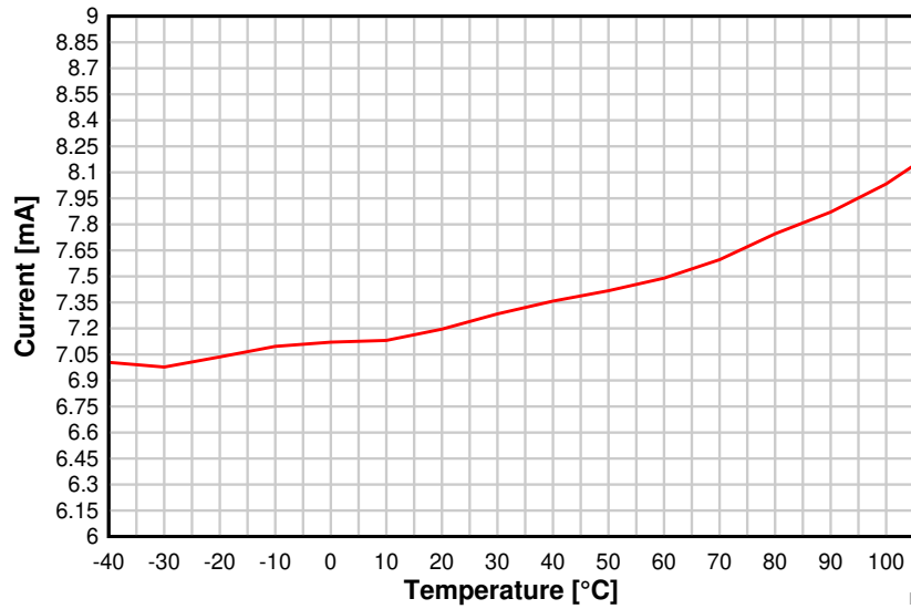
图 8-8. TX Current vs. Temperature (BLE 1 Mbps, 2.44 GHz)
