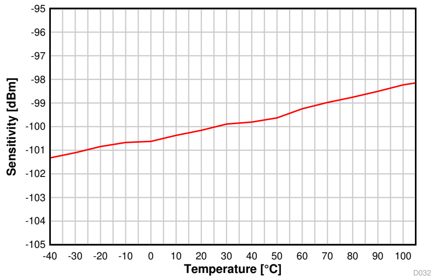
图 8-17. Sensitivity vs. Temperature (250 kbps, 2.44 GHz)
