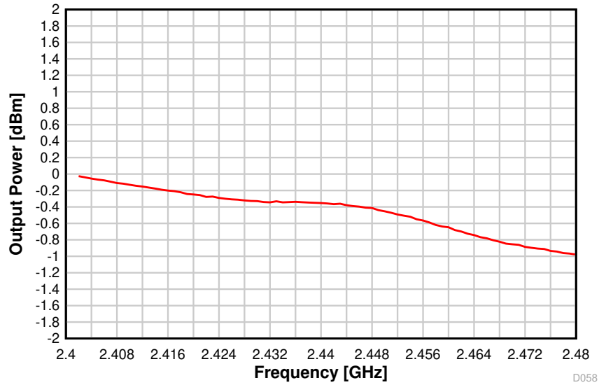
图 8-29. Output Power vs. Frequency (BLE 1 Mbps, 2.44 GHz)
