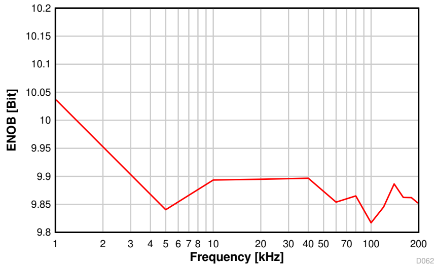
图 8-34. ENOB vs. Sampling Frequency
