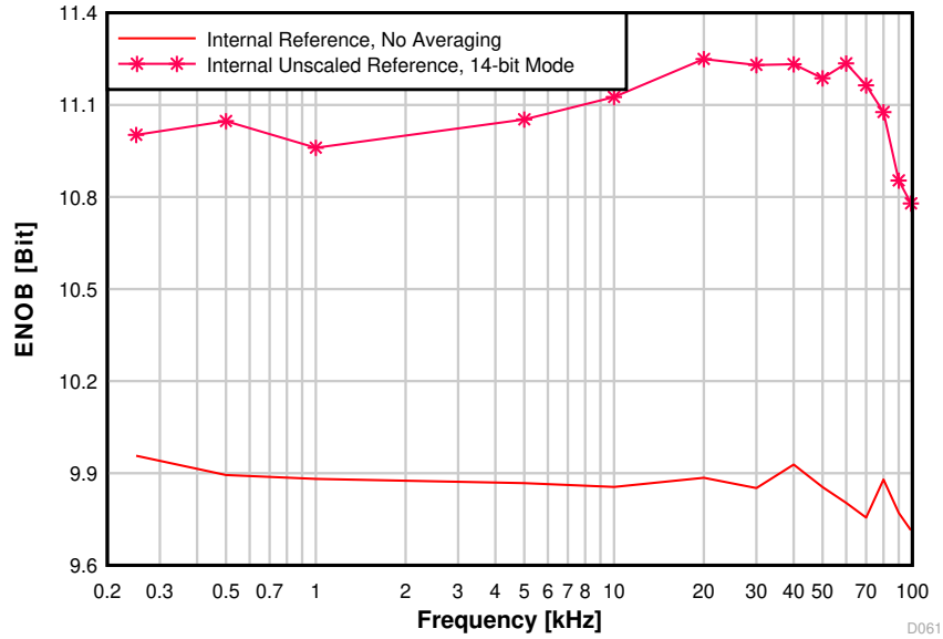
图 8-33. ENOB vs. Input Frequency
