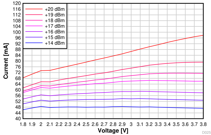
图 8-12. TX Current vs. Supply Voltage (VDD5) (BLE 1 Mbps, 2.44 GHz, +20 dBm PA)
