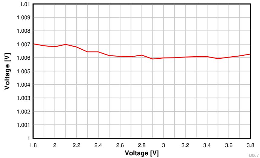
图 8-38. ADC Accuracy vs. Supply Voltage (VDDS)
