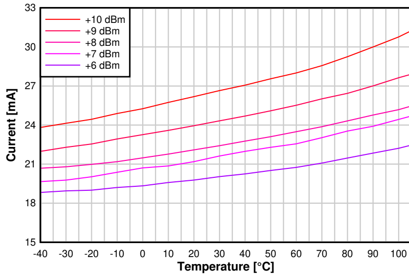
图 8-10. TX Current vs. Temperature (250 kbps, 2.44 GHz, +10 dBm PA)
