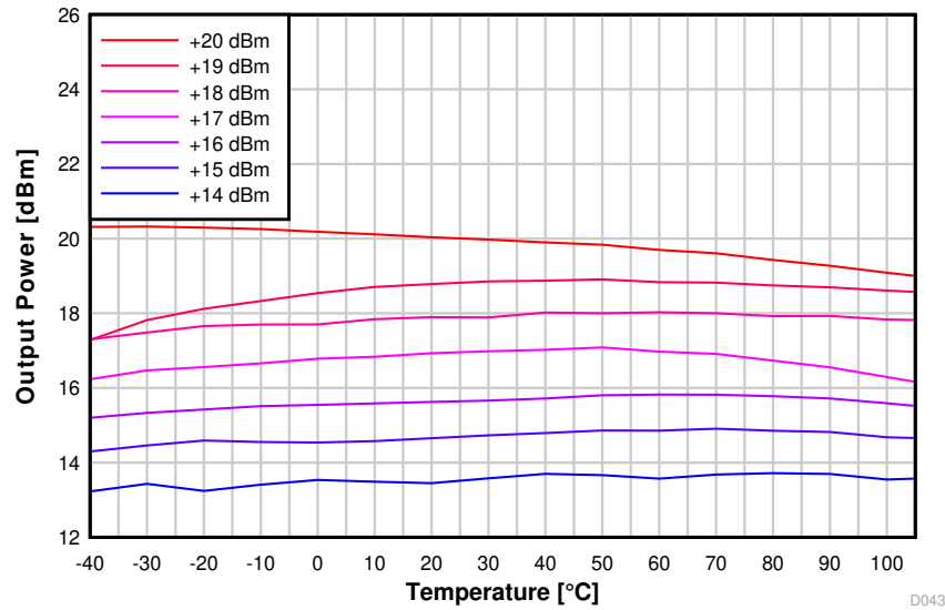
图 8-23. Output Power vs. Temperature (BLE 1 Mbps, 2.44 GHz, +20 dBm PA)
