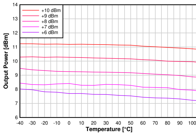
图 8-24. Output Power vs. Temperature (2.44 GHz, +10 dBm PA)
