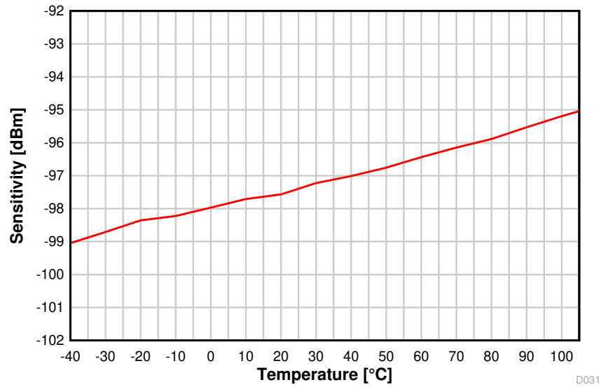
图 8-16. Sensitivity vs. Temperature (BLE 1 Mbps, 2.44 GHz)
