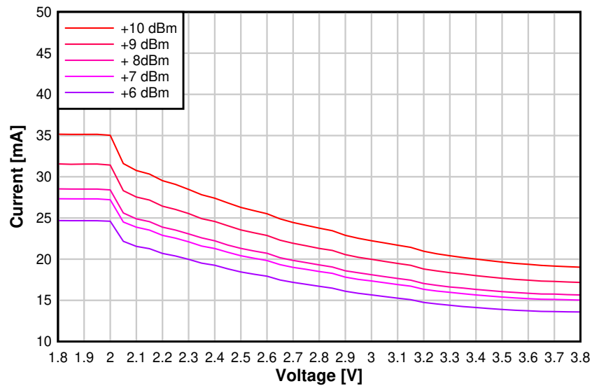
图 8-13. TX Current vs. Supply Voltage (VDD5) (250 kbps, 2.44 GHz, +10 dBm PA)
