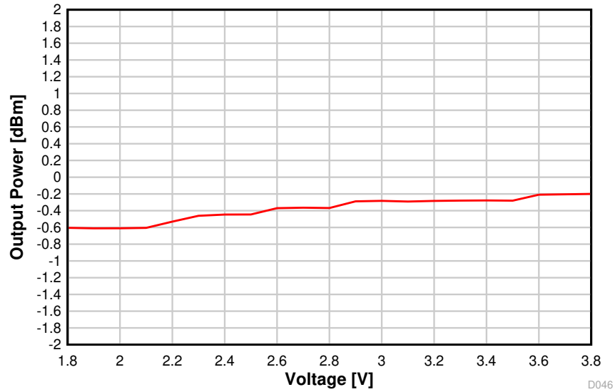
图 8-25. Output Power vs. Supply Voltage (VDD5) (BLE 1 Mbps, 2.44 GHz)
