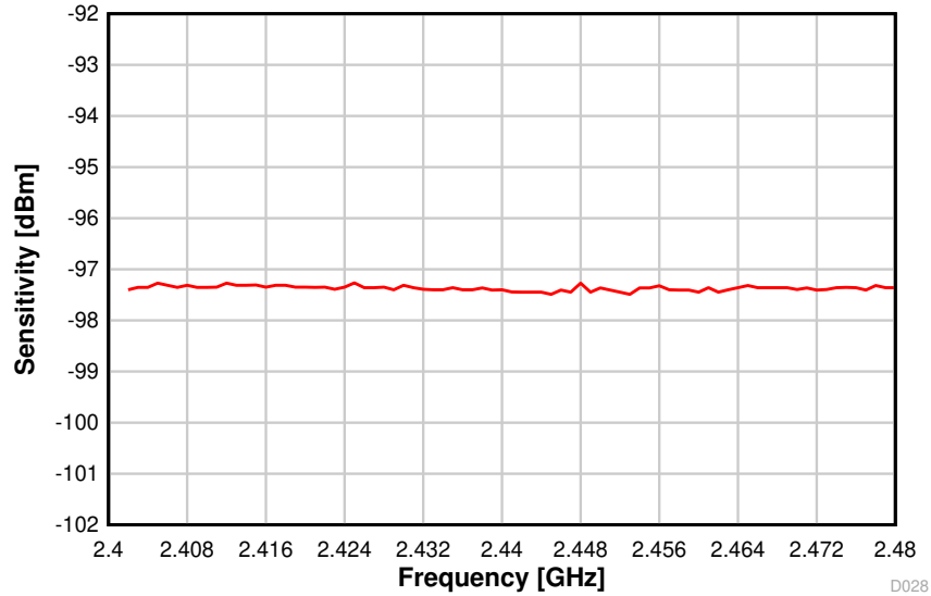
图 8-14. Sensitivity vs. Frequency (BLE 1 Mbps, 2.44 GHz)
