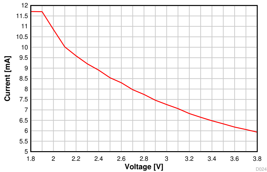
图 8-11. TX Current vs. Supply Voltage (VDD5) (BLE 1 Mbps, 2.44 GHz)
