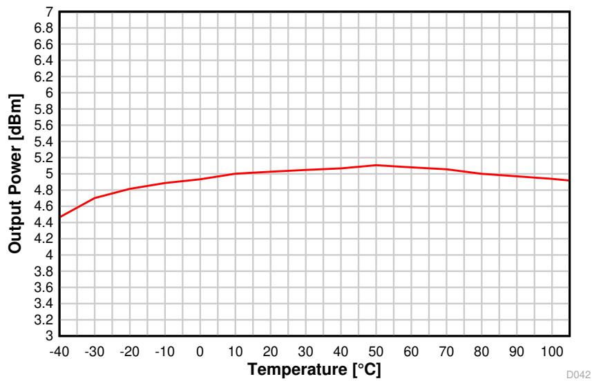
图 8-22. Output Power vs. Temperature (BLE 1 Mbps, 2.44 GHz, +5 dBm)
