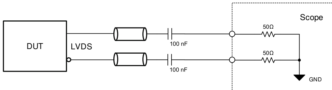
Figure 11. LVDS Output Test Configuration, AC-Coupled
