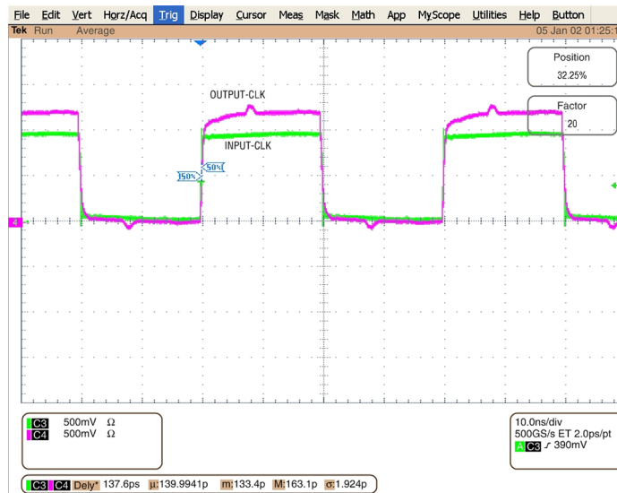
Figure 24. Input/Output Alignment in External Zero Delay Mode for LVCMOS Output
