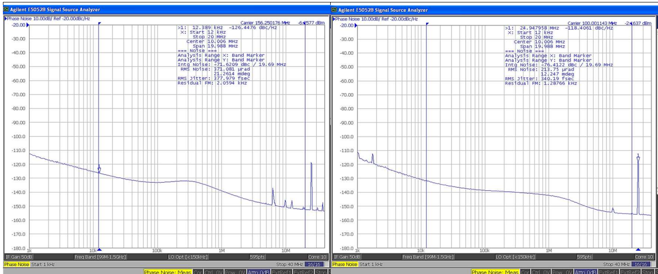
Reference: Crystal Input 25 MHz Closed-Loop Phase Noise from 2.5-GHz VCO 156.25-MHz LVDS
