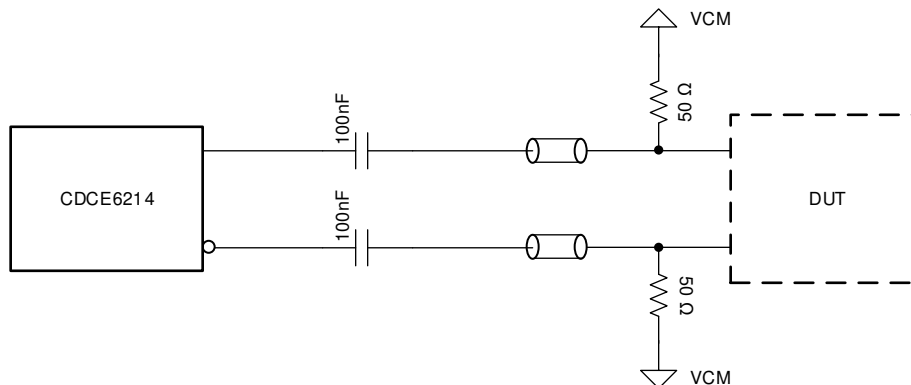
Figure 21. LVDS Output - AC-Coupled
