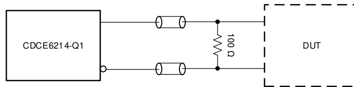
图 8-12. LVDS Output - DC-Coupled. Place 100 Ω close to the DUT
