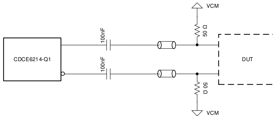
图 8-13. LVDS Output - AC-Coupled
