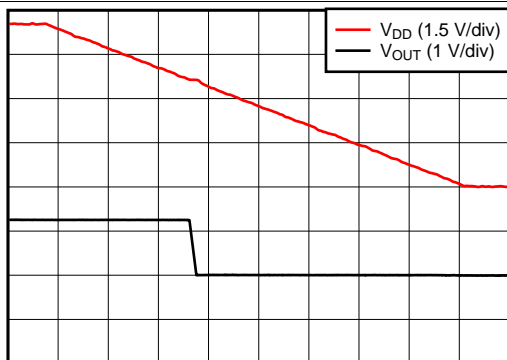
Figure 43. DACx0508C, Clear to Zero Scale
