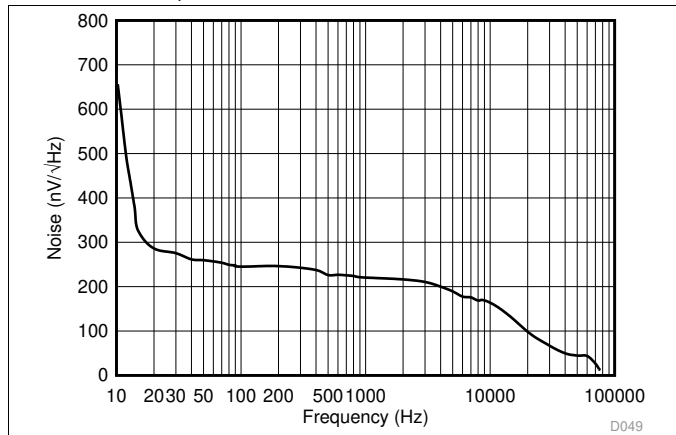
图 51. Internal Reference Noise Density vs Frequency
