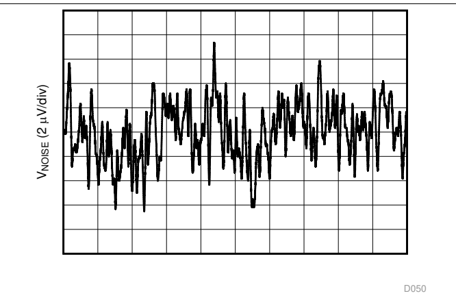
图 52. Internal Reference Noise, 0.1 Hz to 10 Hz
