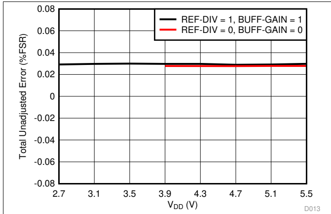
图 15. Total Unadjusted Error vs Supply Voltage
