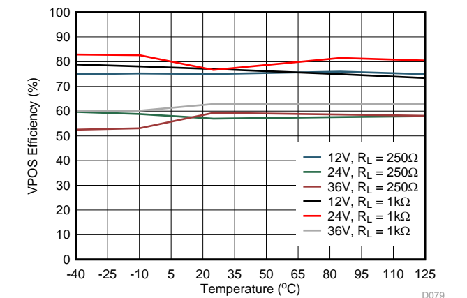
图 81. VPOS Efficiency vs Temperature
