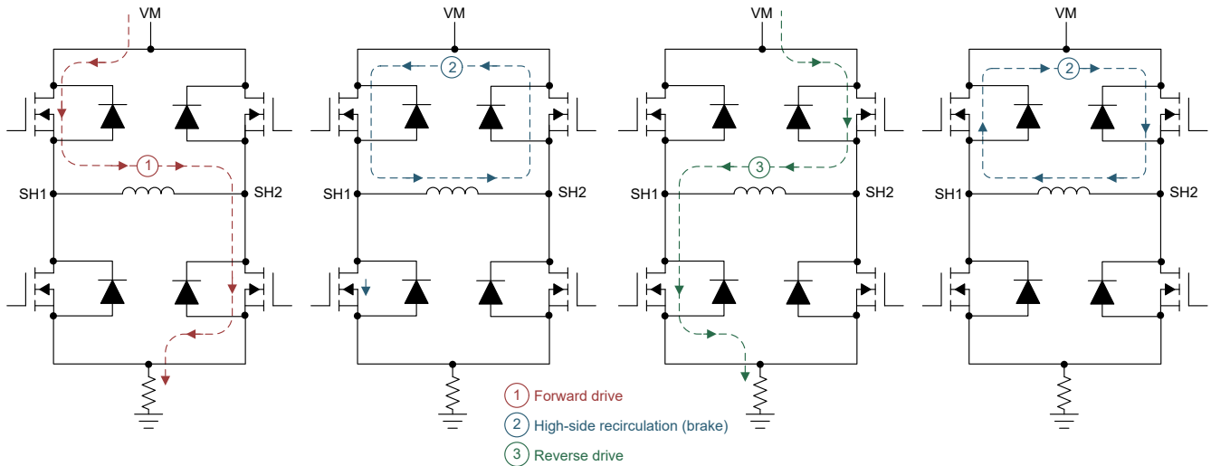
Figure 7-3. Current Paths
