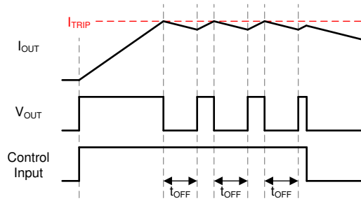
Figure 7-6. Current Regulation
