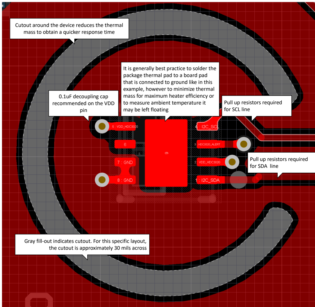
Figure 9-3. HDC302x-Q1 PCB Layout Example
