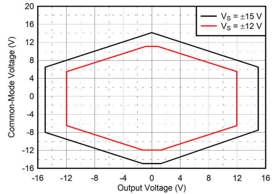
图 8-6. Input Common-Mode Voltage vs Output Voltage G > 10, V_{REF} = 0 \text{ V}
