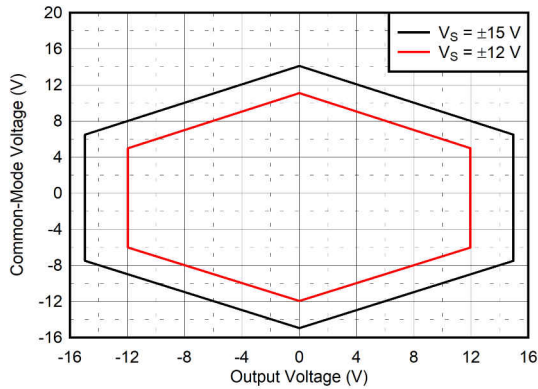
图 8-5. Input Common-Mode Voltage vs Output Voltage G = 1, V_{REF} = 0 \text{ V}
